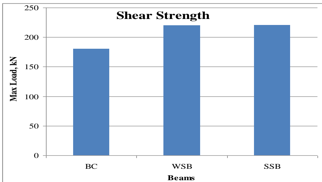
Figure 7: Shear strength of the three tested beams
