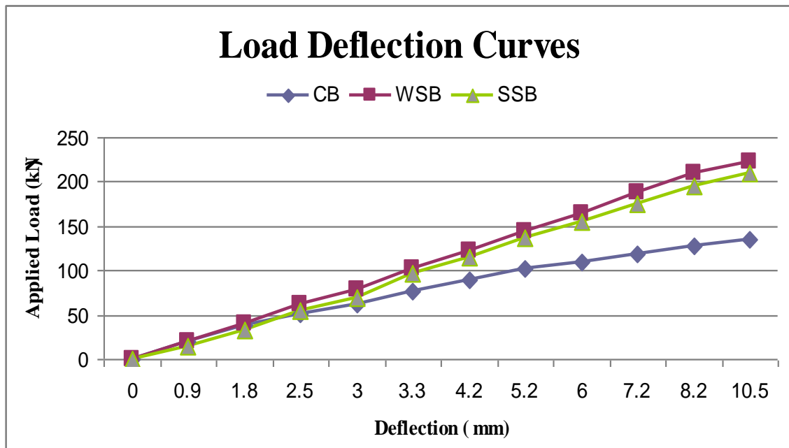
Figure 8: Deflection measured at mid-span as the applied load increases.
