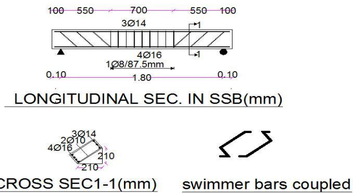
Figure 1: Reinforcement details of the spliced swimmer bars beam, SSB
